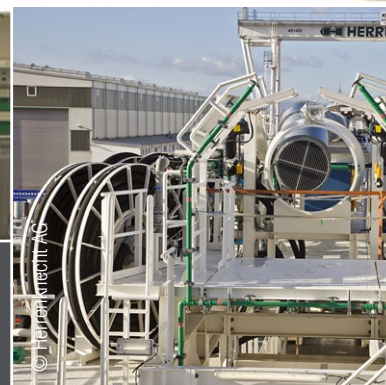
Hose reel during TBM build up for Herrenknecht "Rastatt" - Germany
