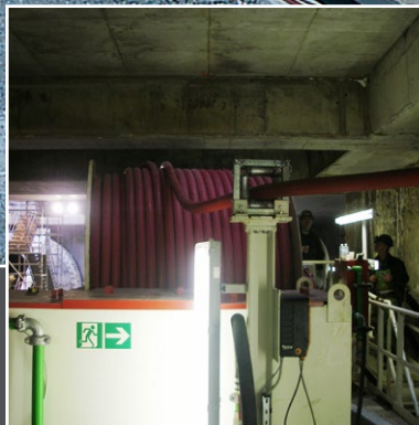
Hydra cable reel feeding power on Tunnel Boring Machine by Herrenknecht
